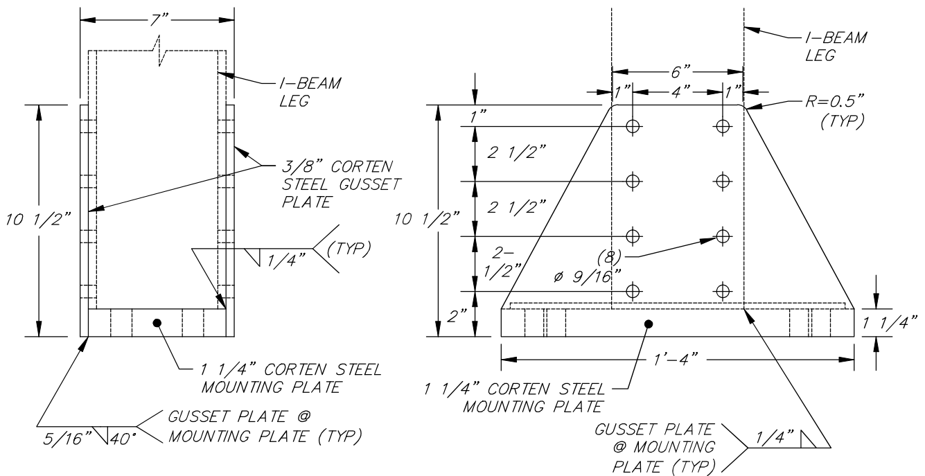
(ST-2) STEEL GUSSET PLATE
