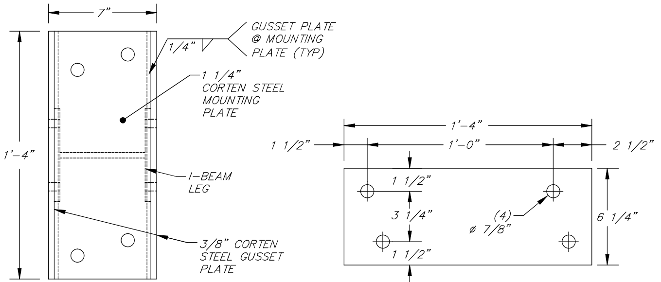
(ST-2) 1 1/4" STEEL MOUNTING PLATE
