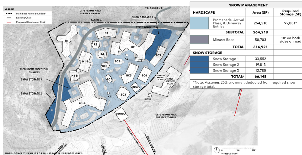
Figure 22 - Parcel A Proposed Snow Management
