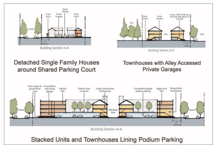
Figure 5-21: Shady Rest Site Development Concept
