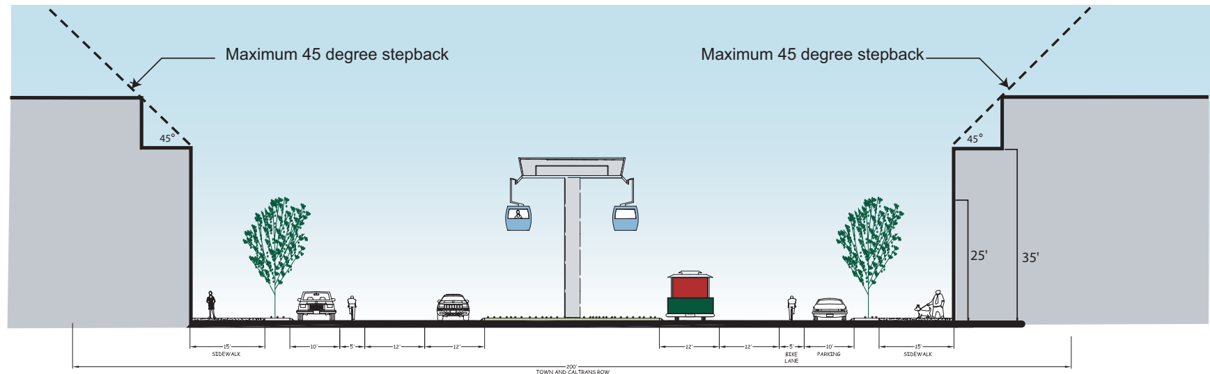
DOWNTOWN SECTION
