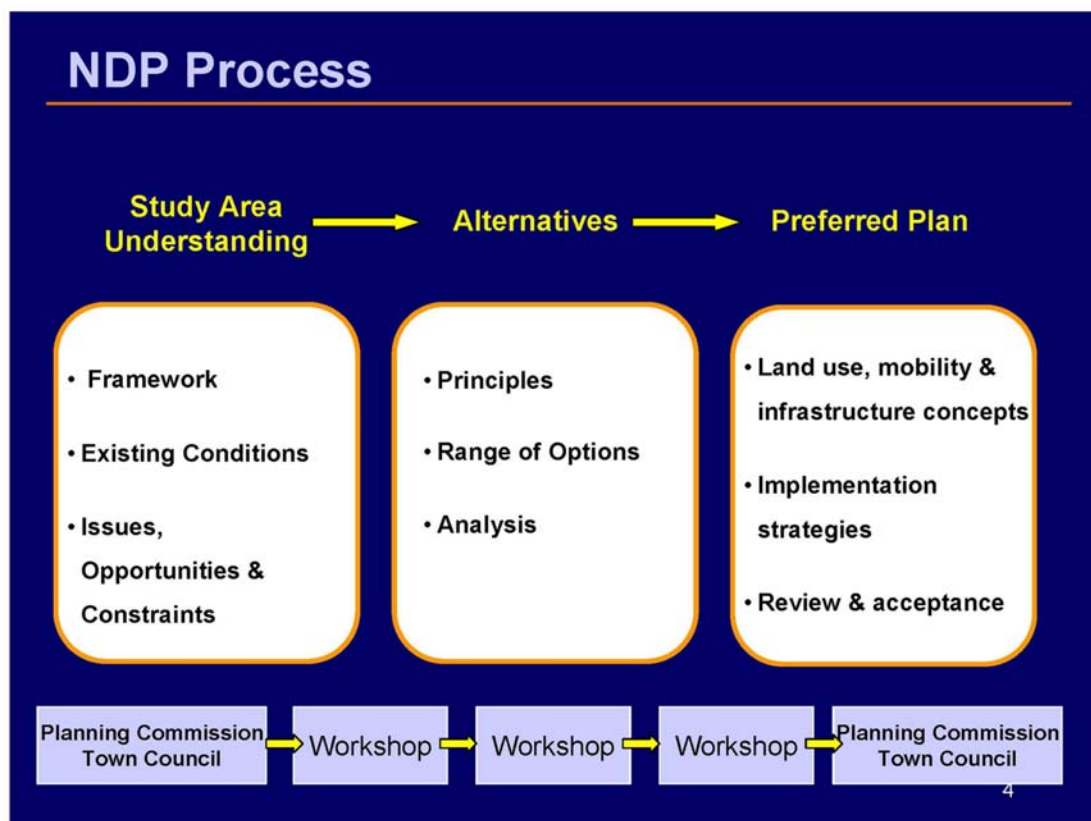
Figure 2-2: NDP Process
