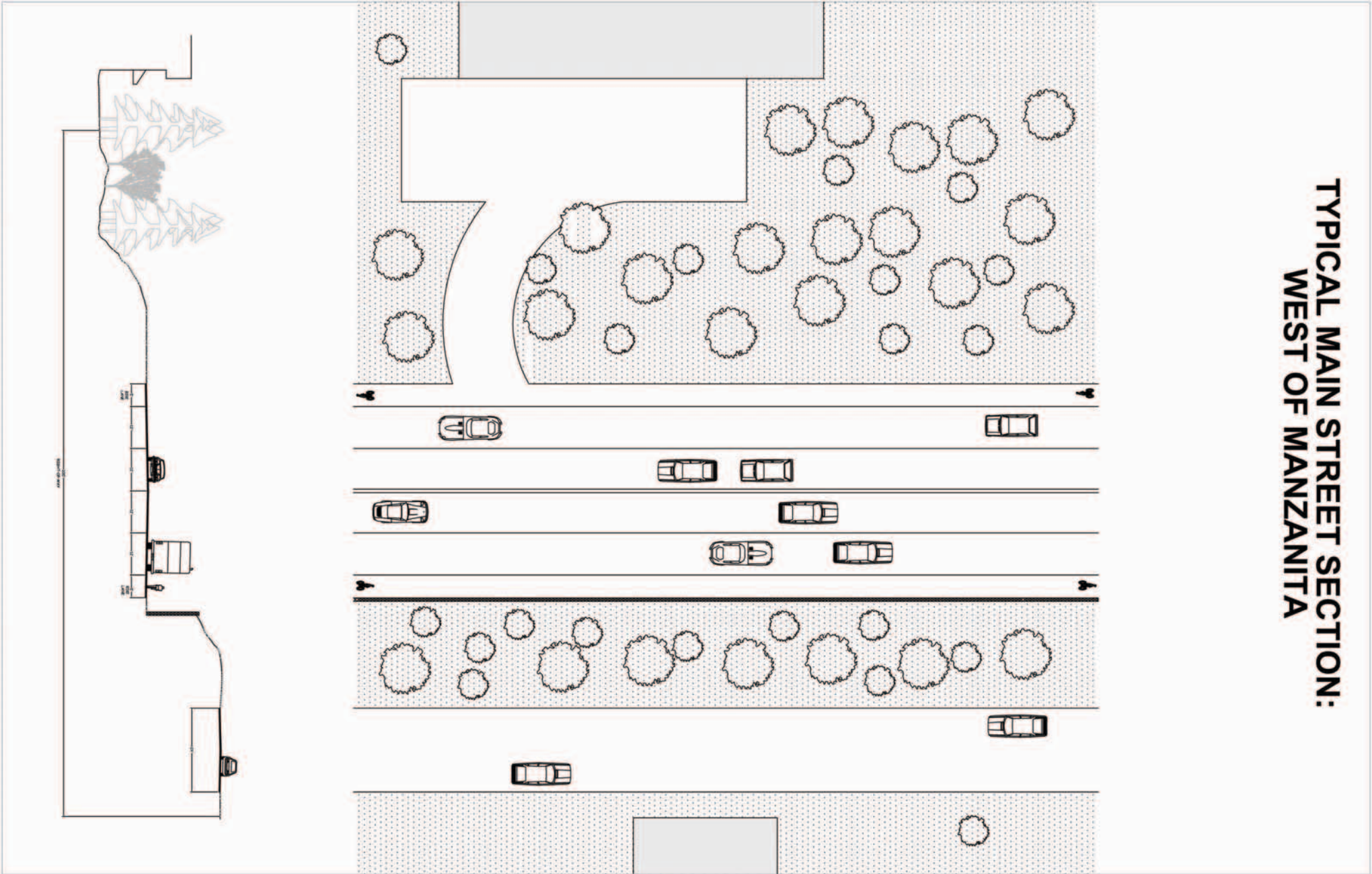
Figure 5-3: Typical Main Street Section, West of Manzanita
