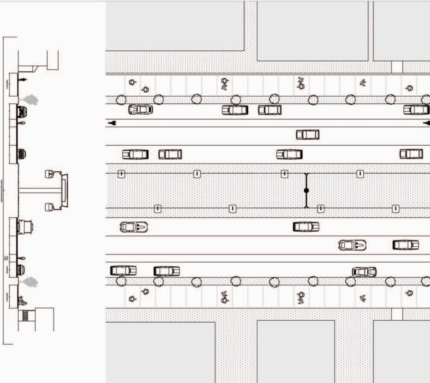
Figure 5-2: Downtown Cross Section
